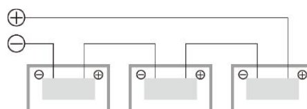
Example of connection in series
